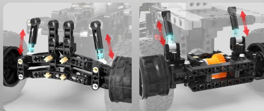
Front Suspension
